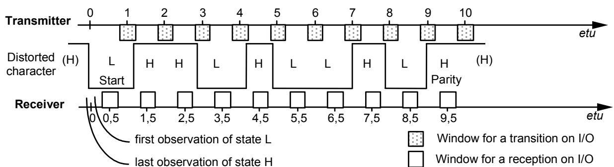
Figure 8 — Character timings
