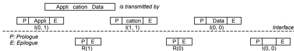
Figure 23 — Chaining function
