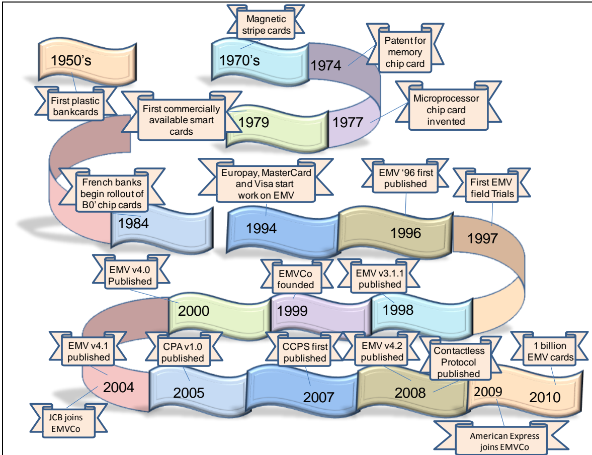
Figure 1: EMV Timeline
