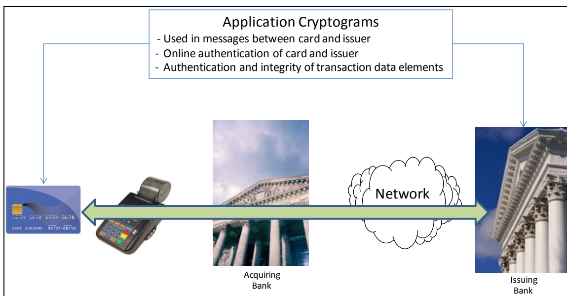
Figure 5: Application Cryptograms
